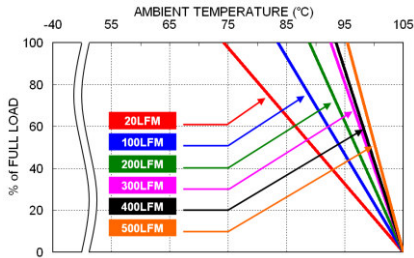
RHK10-110S05W Derating Curve
